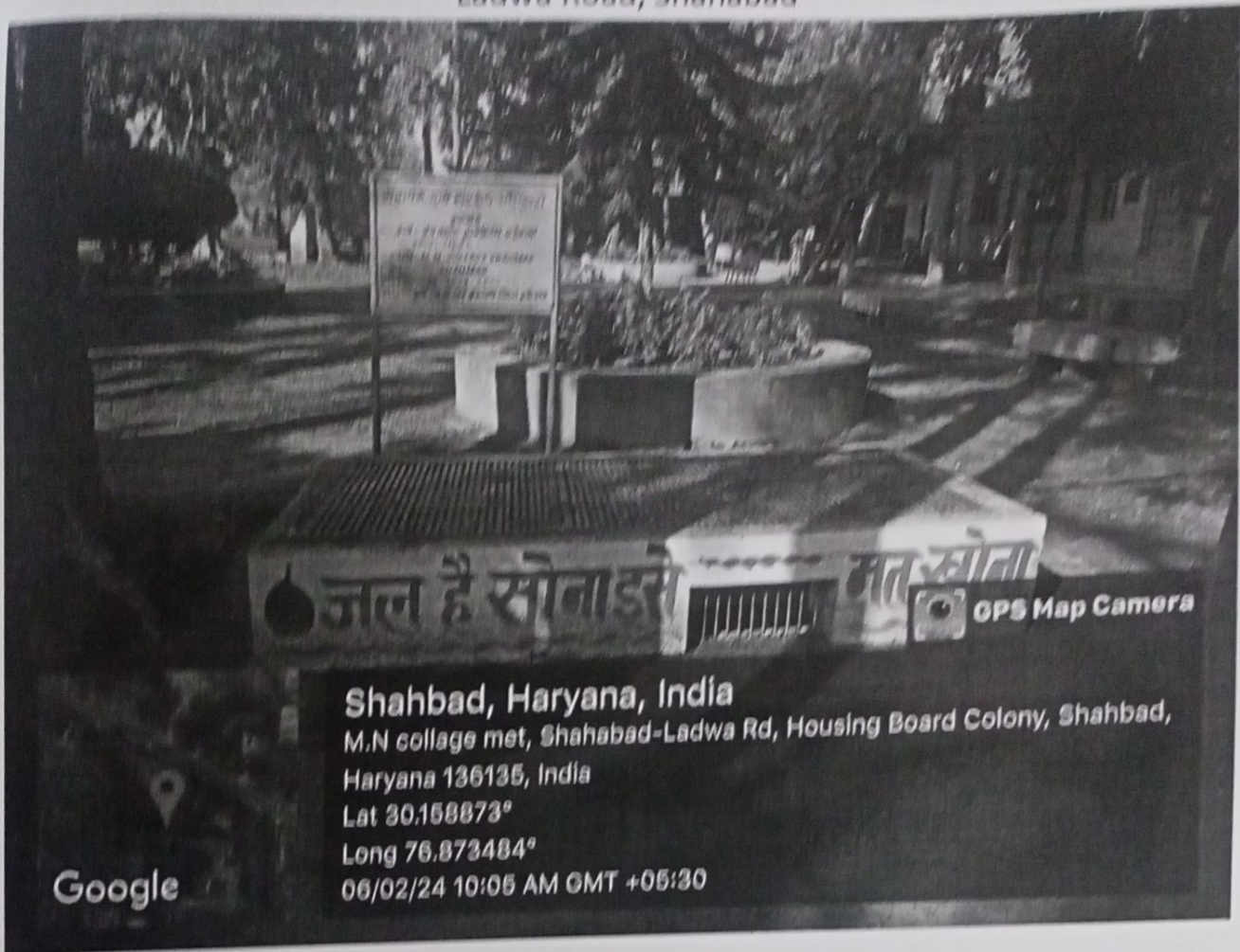
Rain Water Harvesting and Ground water recharge System in Lawn-2
